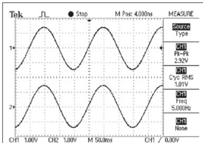
FIGURE 6: Sine wave performance at 5Hz.
