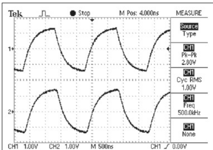
FIGURE 11: Square wave performance at 500kHz.
