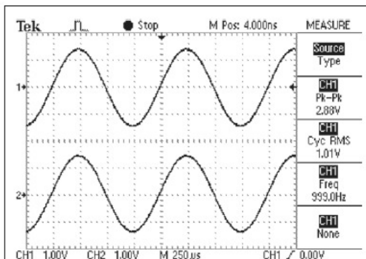
FIGURE 7: Sine wave performance at 1kHz.
