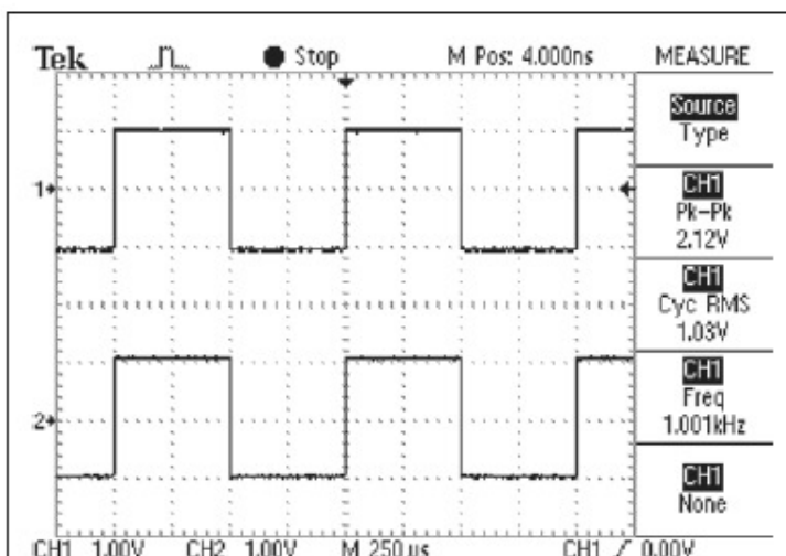
FIGURE 10: Square wave performance at 1kHz.
