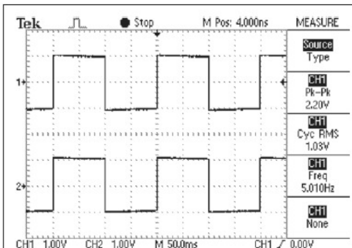
FIGURE 9: Square wave performance at 5Hz.
