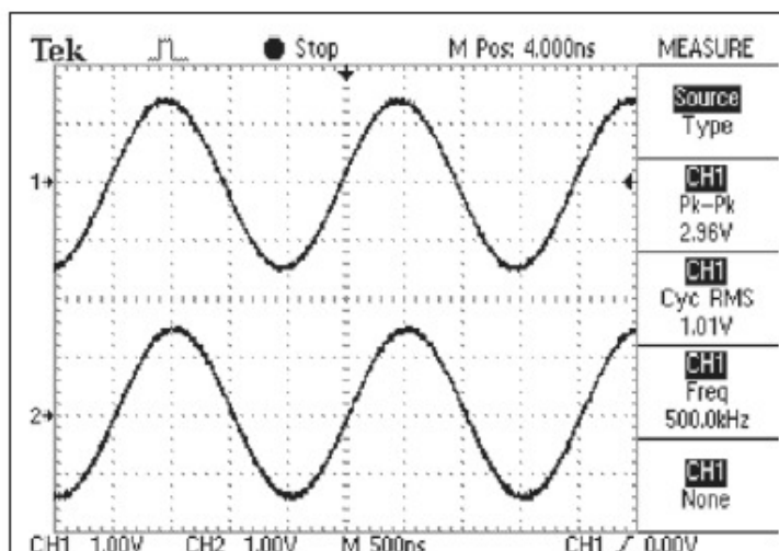
FIGURE 8: Sine wave performance at 500kHz.
